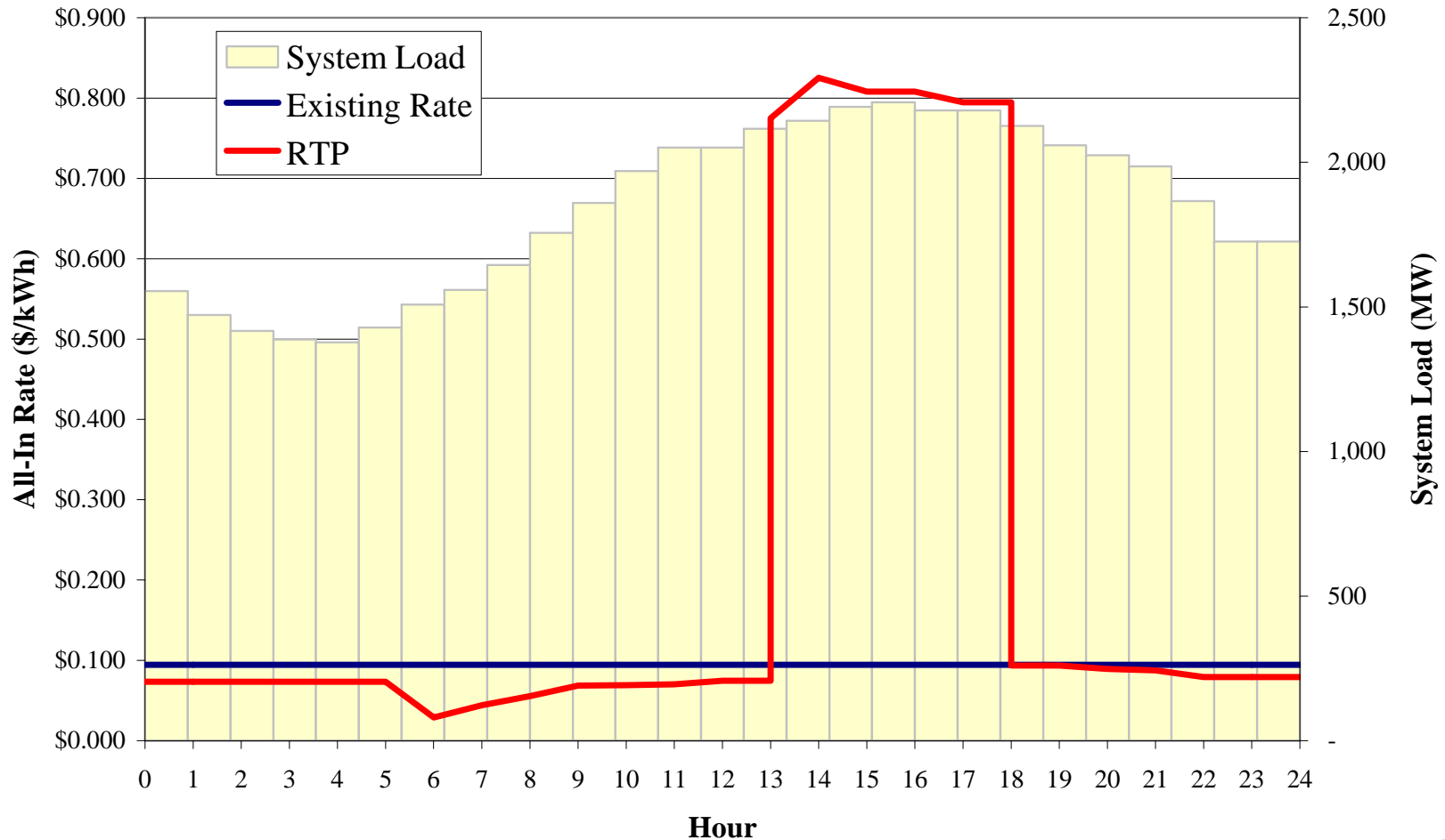
Illustrative RTP on a Critical Day - Residential
