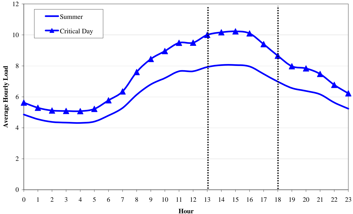
Small General Service Load Profile (2007)
