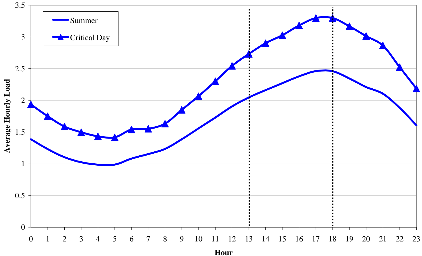
Residential Load Profile (2007)
